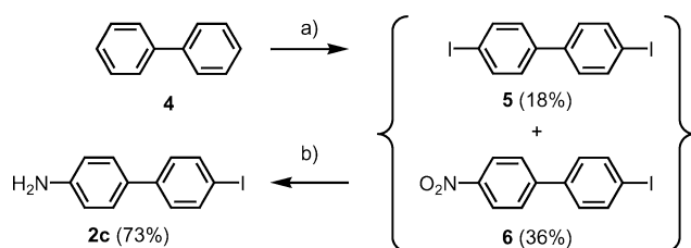
Scheme 3. Two-step synthesis of biphenyl derivative 2c . Reagents and conditions: a) 1 equiv. I 2 , 2.5 equiv. concd. HNO 3 , 5 equiv. concd. H 2 SO 4 , AcOH, 110 °C, 2 h; b) Zn, HCl, EtOH, 78 °C, 1 h.
