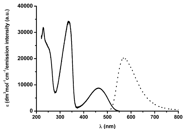
Figure 3. The absorption (solid) and emission (dotted) spectra of 3d . The absorption spectrum is shown in molar absorption units; the emission spectrum (excited by 350 nm light) is given in arbitrary units.
