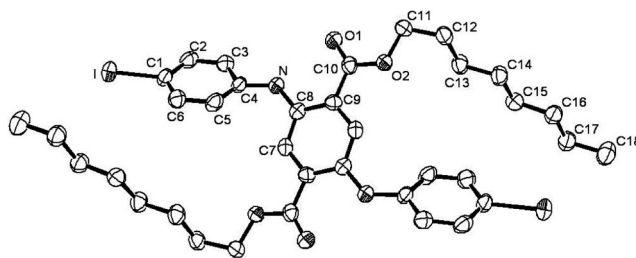
Figure 2. ORTEP representation of the structure of compound 3d in the solid state.
