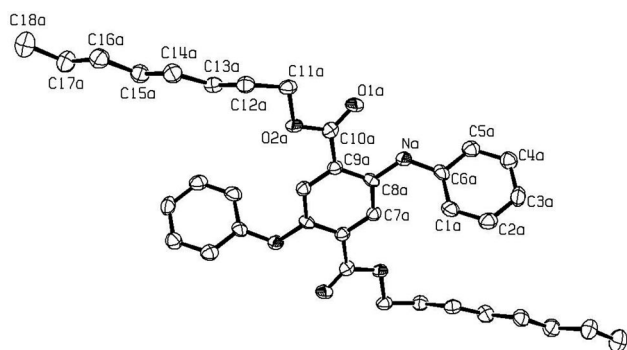
Figure 1. ORTEP view of one (molecule a) of the two independent molecules of compound 3b in the unit cell.
