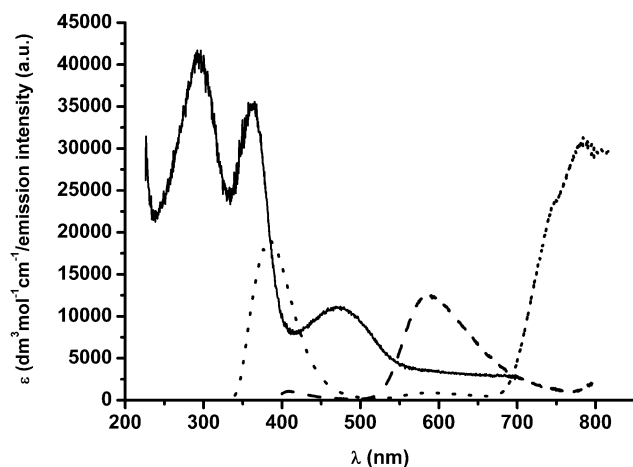
Figure 4. The absorption (solid) and emission [excited at 350 nm (dashed) and 300 nm (dotted)] spectra of 3r . The absorption spectrum is shown in molar absorption units and the emission spectra in arbitrary units.
