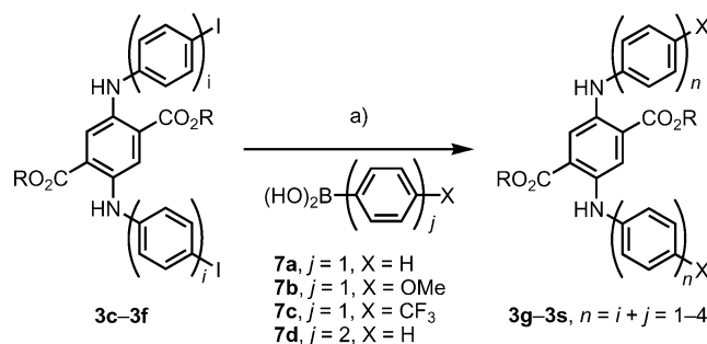
Scheme 4. Synthesis of fluorescence materials 3g–3s by Suzuki cross-coupling reaction. For yields and substituents R and X, see Table 2. Reagents and conditions: a) 5 mol-% [Pd(PPh 3 ) 4 ], 4 equiv. Na 2 CO 3 , toluene/EtOH/H 2 O (1:1:1.5), reflux, 16 h.
