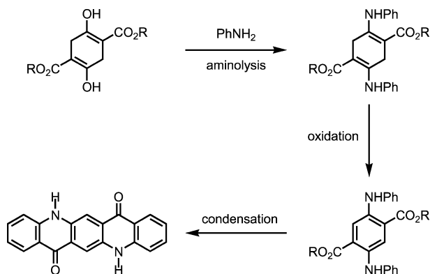
Scheme 1. Industrial synthesis of quinacridone pigments from succinyl succinates.
