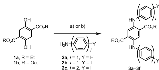
Scheme 2. Synthesis of fluorescence materials 3a–3f by oxidative aminolysis of succinyl succinates 1 . For yields and substituents R and Y, see Table 1. Reagents and conditions: a) cat. HCl, air, toluene, 60 °C, 2 d (for 3a , 3b , 3d ), 16 h (for 3c ); b) air, AcOH, 100 °C, 16 h (for 3e , 3f ).
